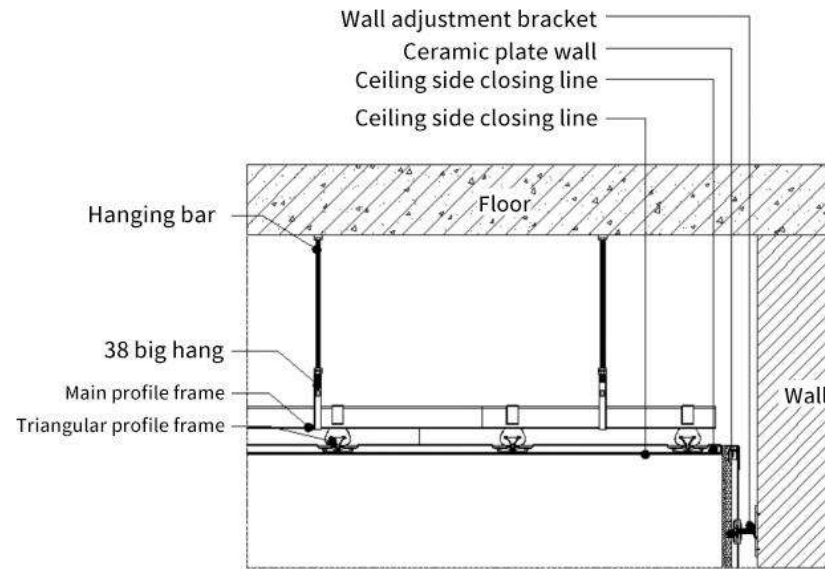
Node at the junction of ceiling and wall
