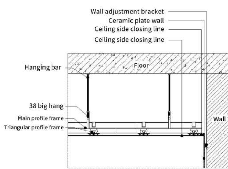
Node at the junction of ceiling and wall
