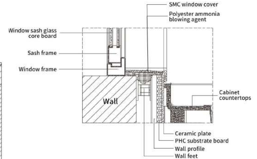
SMC window cover installation node
