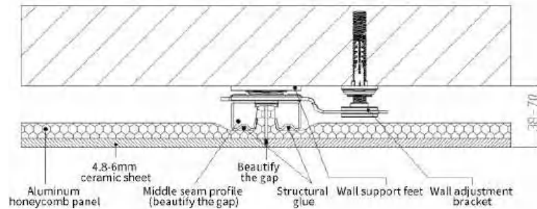
PHC wall profile node -center seam (beautify the gap)
