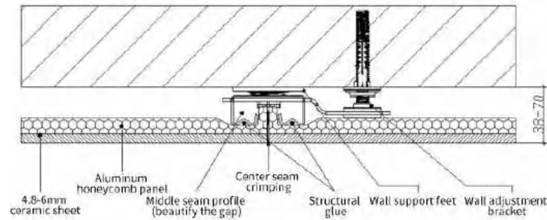
PHC wall profile node -center seam (beautify the gap)
