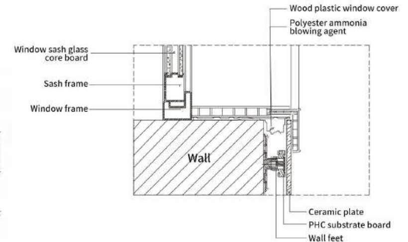
Wood plastic window cover installation node
